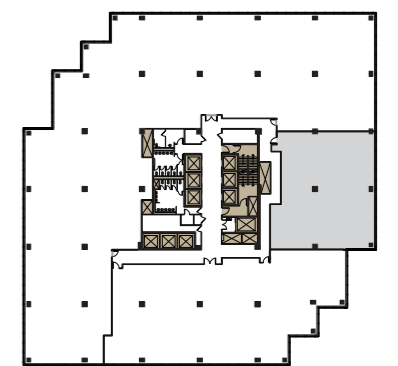
8TH FLOOR KEY PLAN
